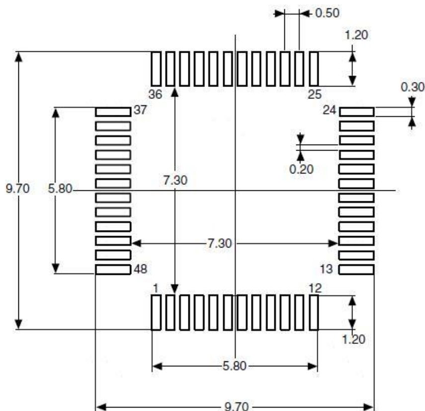
Figure 19 LQFP48, 7x7mm Welding Layout Recommendations
