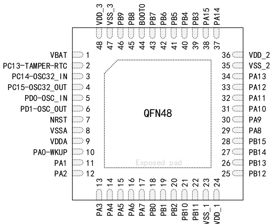
Figure 3 Distribution Diagram of APM32F402xB Series QFN48 Pins
