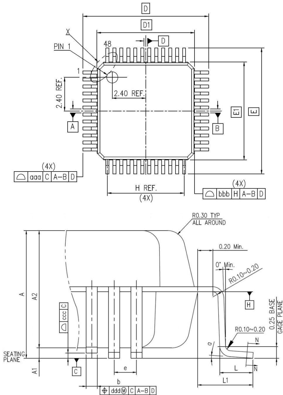
Figure 18 LQFP48 Package Diagram
