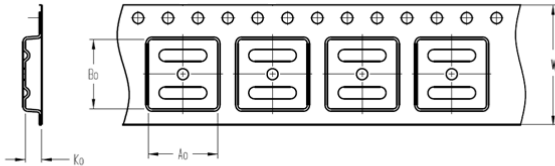
Figure25 Reel Packaging Specification Drawing
