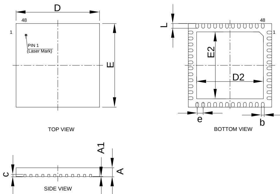
Figure 20 QFN48 Package Diagram
